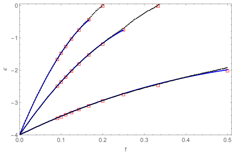
Figure 7: The position of the LLs \epsilon_n^{\text{GN}}(f) obtained from the Roth-Gao-Niu rule (blue line) fits very well the field dependence of the average energy of the Landau bands (black dots) obtained from the Hofstadter spectrum. The position of the middle of the bands when f = 1/q is also plotted (red squares). These fits work perfectly well up to the maximal flux f_{\max}(n) = \frac{1}{2(n+1)} (where n = 0, 1, 2, \dots is the Landau index) and start to deviate beyond that.
