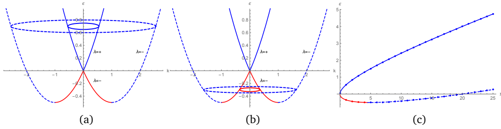
Figure 4: Rashba model. (a) and (b): Energy spectrum \epsilon_\lambda(k) = \frac{k^2}{2m} + \lambda k [ \epsilon is in units of m ] as a function of the wavevector k [in units of m ]. The dispersion relation is isotropic in (k_x, k_y) space. The inner branches are plotted in full lines and the outer branches in dashed lines. The electron-like branches are in blue and the hole-like branches are in red. Fermi circles are also indicated for the case of positive (a) or negative energy (b). (c) LLs: energy \epsilon_{\bar{n},\lambda} [in units of m ] as a function of the Landau index \bar{n} = n + \frac{1-\lambda}{2} between 0 and 25 for \lambda = + (blue) and between 1 and 25 for \lambda = - (red for hole-like and dashed blue for electron-like LLs). The magnetic field is fixed such that \frac{2\pi B}{m^2} = 0.1 and we considered the case \tilde{g} = 0 .
