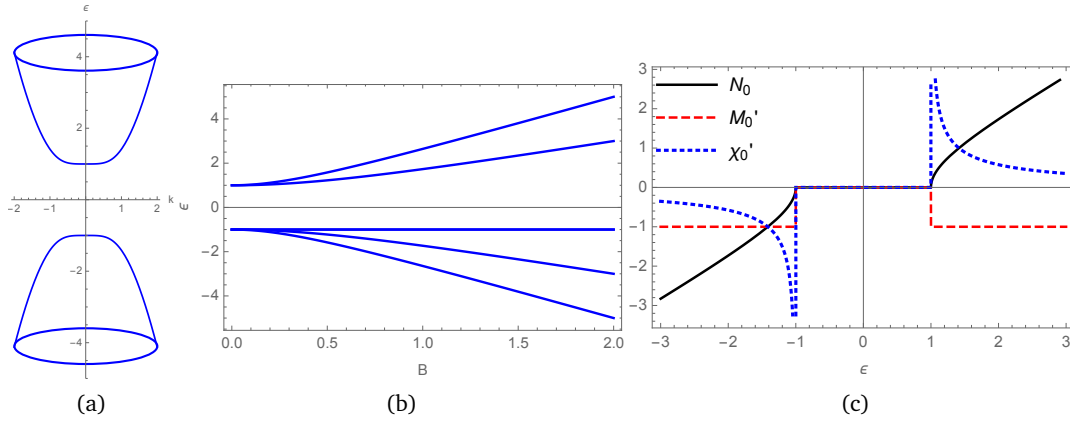
Figure 2: Gapped graphene bilayer. (a) Dispersion relation in zero field: energy \epsilon_\lambda(k) = \lambda \sqrt{\left(\frac{k^2}{2m}\right)^2 + \Delta^2} [in units of \Delta ] as a function of the wavevector k [in units of \sqrt{2m\Delta} ]. (b) Landau levels: energy \epsilon_{n,\xi,\lambda} [in units of \Delta ] as a function of the field B [in units of \frac{m\Delta}{2\pi} ] for different values of the Landau index \bar{n} = n + 1 + \lambda\xi = 2, 3 for \lambda = + and \bar{n} = 0, 1, 2, 3 for \lambda = - (here we consider a single valley \xi = + ). (c) Integrated density of states (IDoS) N_{0,\xi} [black line, in units of \frac{m\Delta}{2\pi} ], derivative of the magnetization M'_{0,\xi} [red dashed line] and derivative of the susceptibility \chi'_{0,\xi} [blue dotted line, in units of \frac{\pi}{2m\Delta} ] as a function of energy \epsilon [in units of \Delta ].
